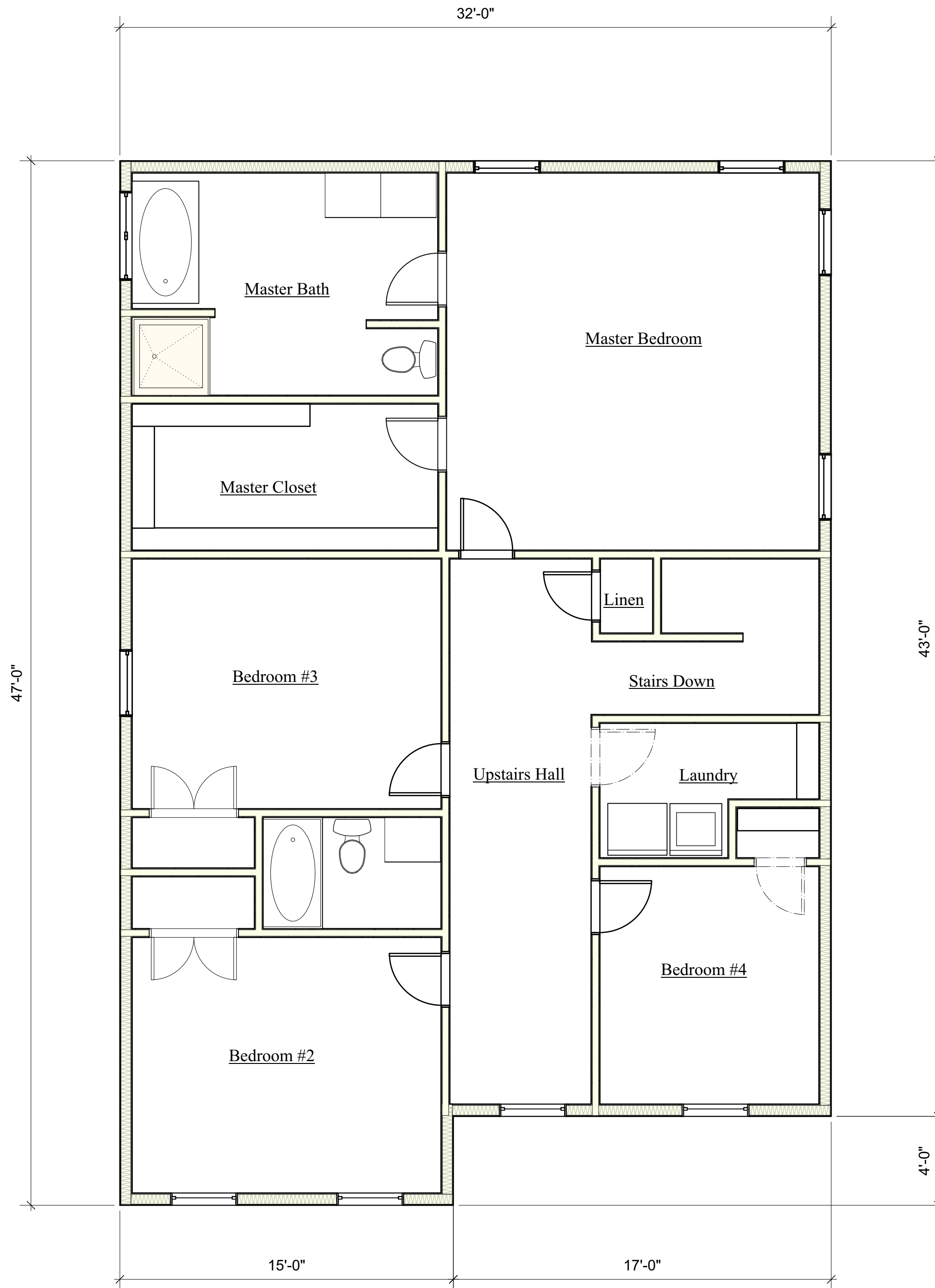
7 2nd Floor Scale: 1/4" = 1'-0"
