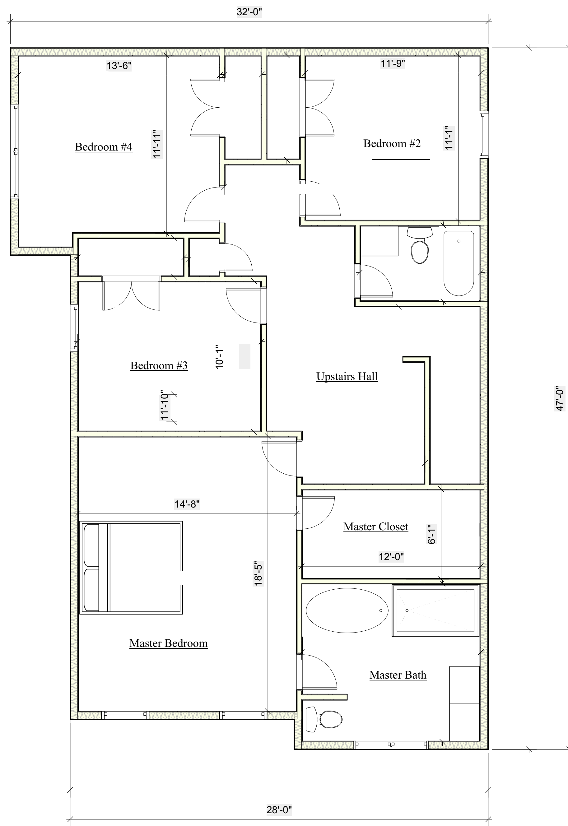
2nd Floor
