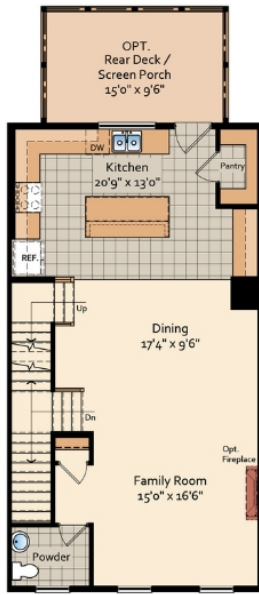
FIRST FLOOR PLAN ELEVATION #1 & #2 Brochure
