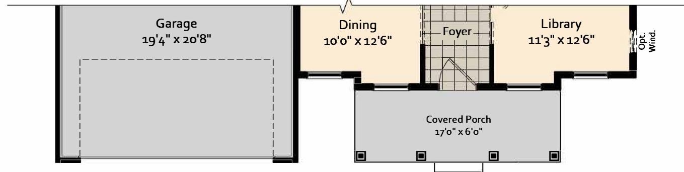
FIRST FLOOR PLAN ELEVATION #2 Brochure
