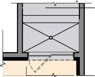
OPT. WIDE AREAWAY PARTIAL PLAN Brochure
