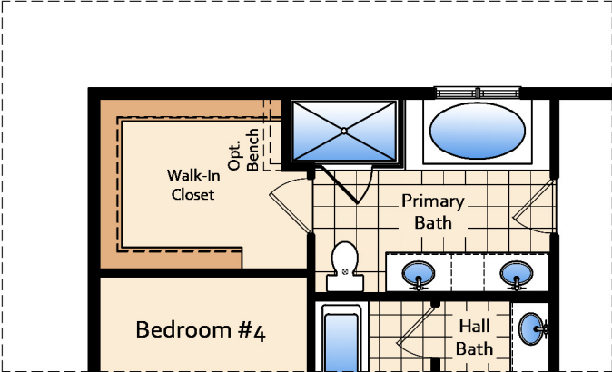
OPT. DELUXE PRIMARY BATH PARTIAL PLAN Brochure
