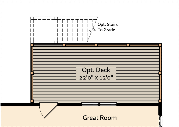
OPT. DECK PARTIAL PLAN Brochure
