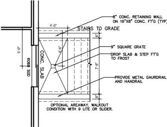
BROCHURE OPT. AREAWAY (EAST)
