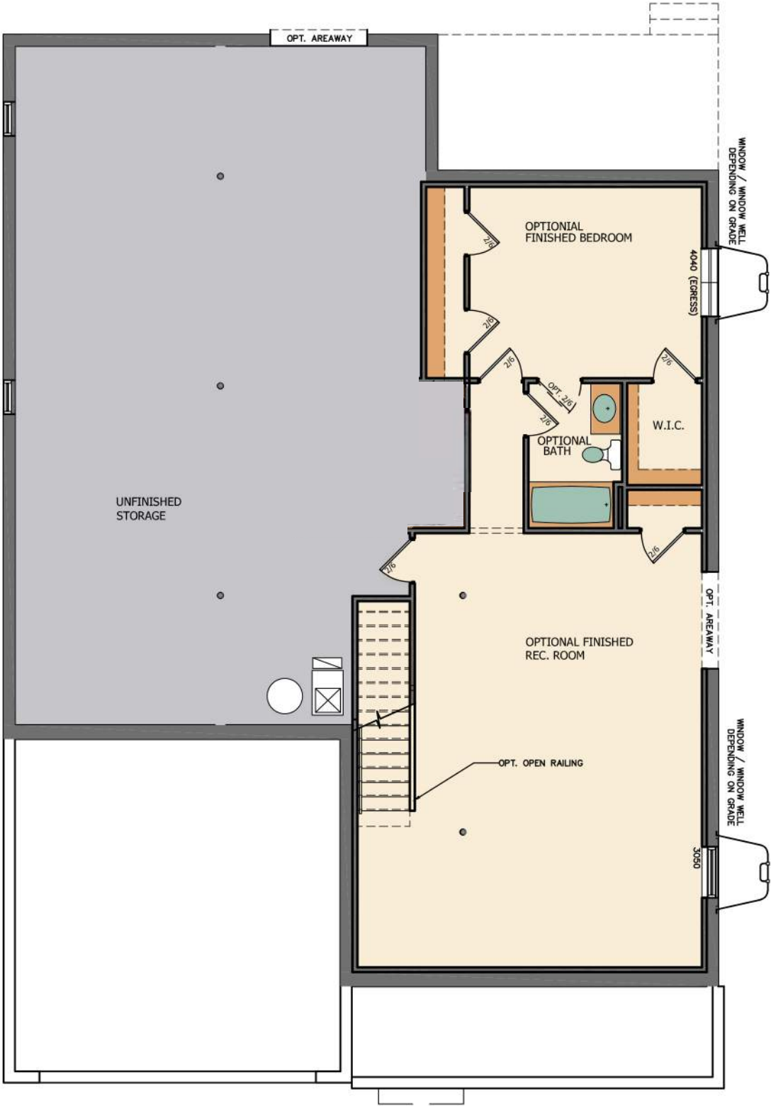
BROCHURE OPT. 8' BASEMENT PLAN
