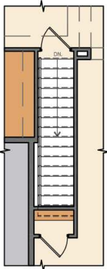
STAIR TO OPT. 9' BSMT PARTIAL PLAN
