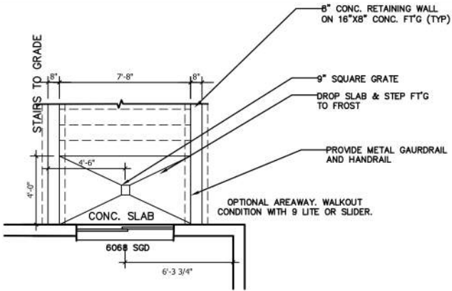
BROCHURE OPT. AREAWAY (NORTH)
