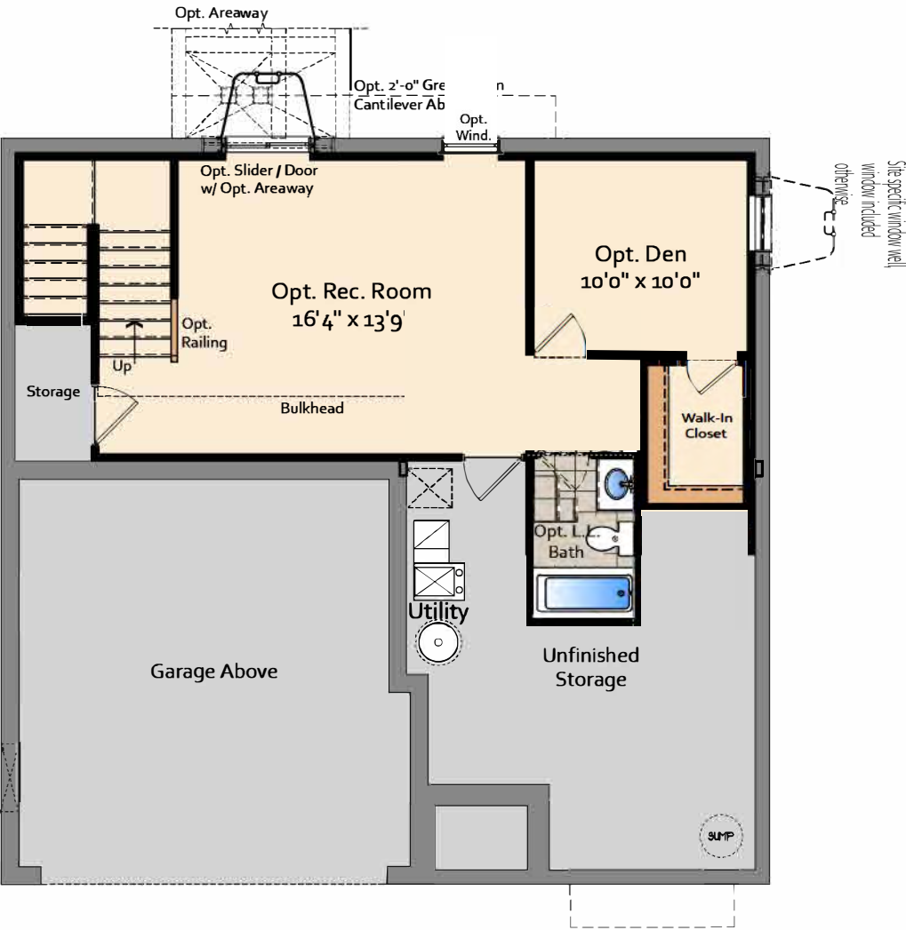
OPT. FINISHED LOWER LEVEL PLAN ELEVATION #1 Brochure
