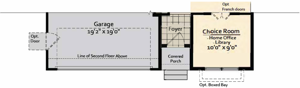
PARTIAL - FIRST FLOOR PLAN ELEVATION #3 Brochure
