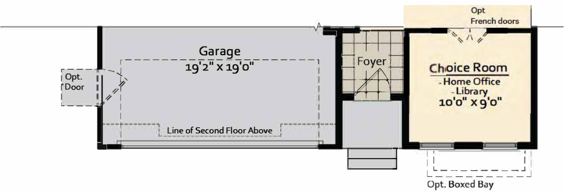
PARTIAL - FIRST FLOOR PLAN ELEVATION #2 Brochure
