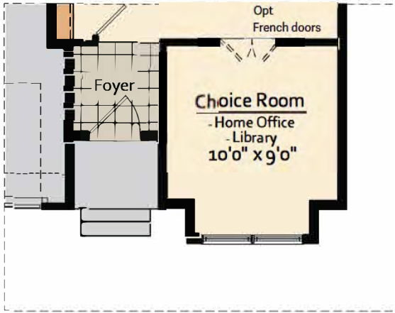
OPT. BOXED BAY PARTIAL PLAN Brochure
