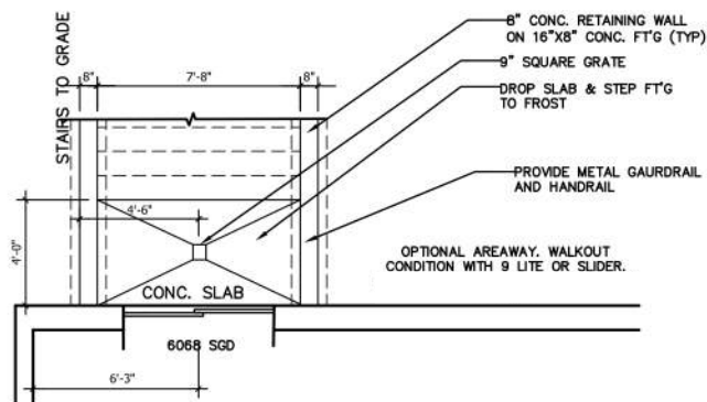
BROCHURE OPT. AREAWAY
