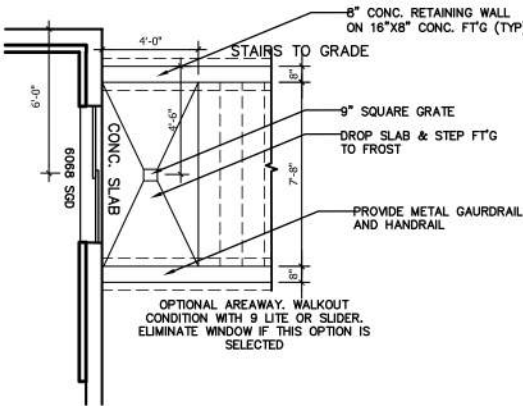
BROCHURE OPT. AREAWAY
