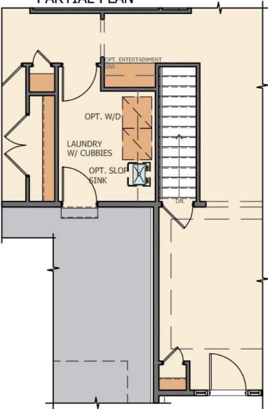
BROCHURE STAIR TO OPT. BASEMENT PARTIAL PLAN
